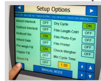
Allen Bradley Control Panel
